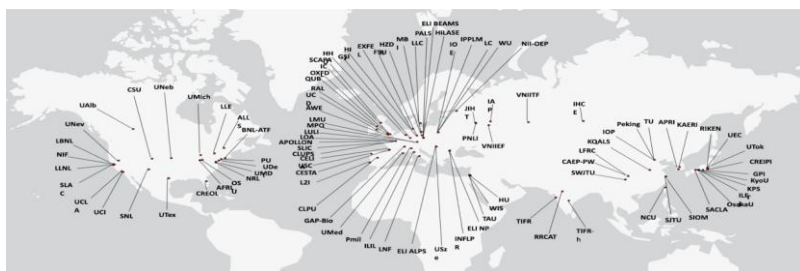
Figure 1. World map of laser with peak power >100 TW, tratto da "Gerard Mourou: Nobel Lecture: Extreme light physics and application", Rev. Mod. Phys. , 91 , 030501 (2019).
